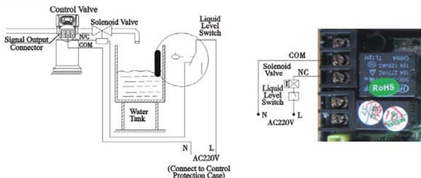
Figure 3-1 Wring of Solenoid Valve on Outlet
