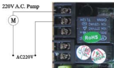
Figure 3-7Wiring of Booster Pump on Inlet
