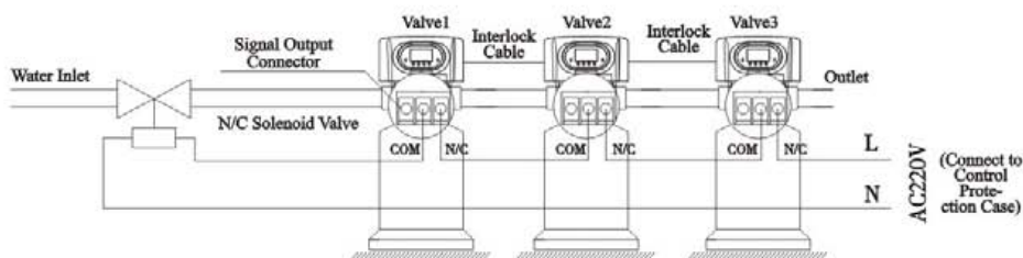
Figure 3-4 Wiring of Solenoid Vale in Inlet
